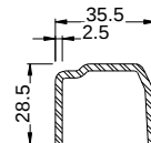
202780 I_x \text{ (cm}^4\text{)} = 3,79 I_y \text{ (cm}^4\text{)} = 1,59
